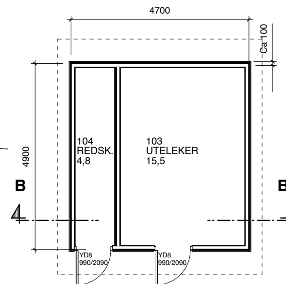
PLAN BOD B
